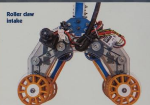
Low scoring
