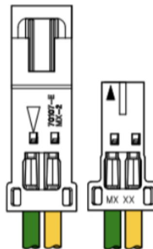
MOLEX SL USED FOR CAN, OTHER ROBUST LOW CURRENT CONNECTIONS
